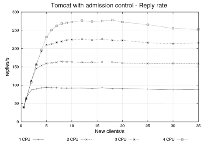
Figure 5. Tomcat with admission control throughput with different number of processors
