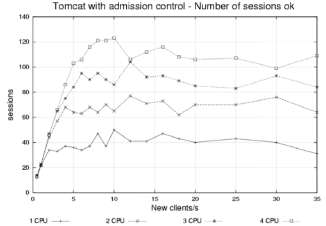
Figure 7. Sessions completed by Tomcat with admission control with different number of processors
