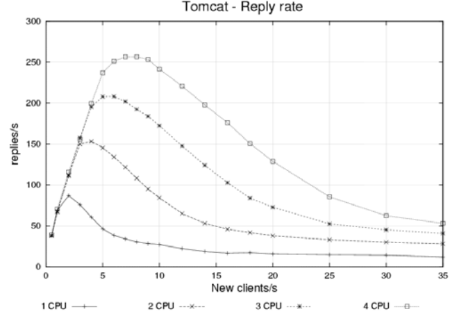
Figure 2. Original Tomcat throughput with different number of processors
