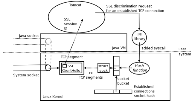
Figure 1. SSL connections differentiation mechanism
