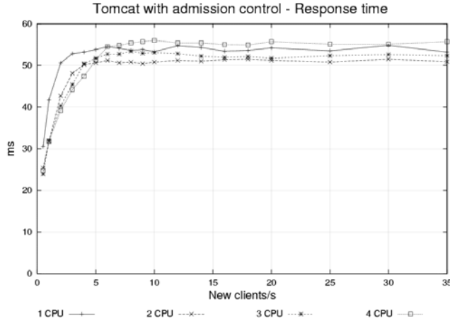
Figure 6. Tomcat with admission control response time with different number of processors
