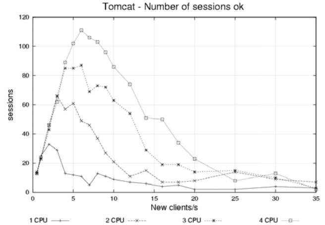
Figure 4. Completed sessions by original Tomcat with different number of processors
