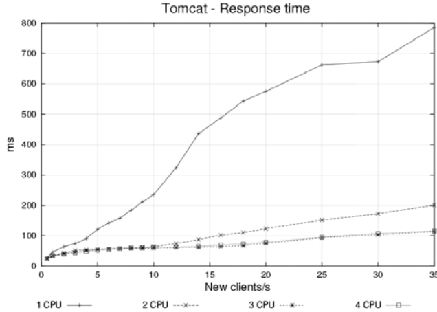
Figure 3. Original Tomcat response time with different number of processors
