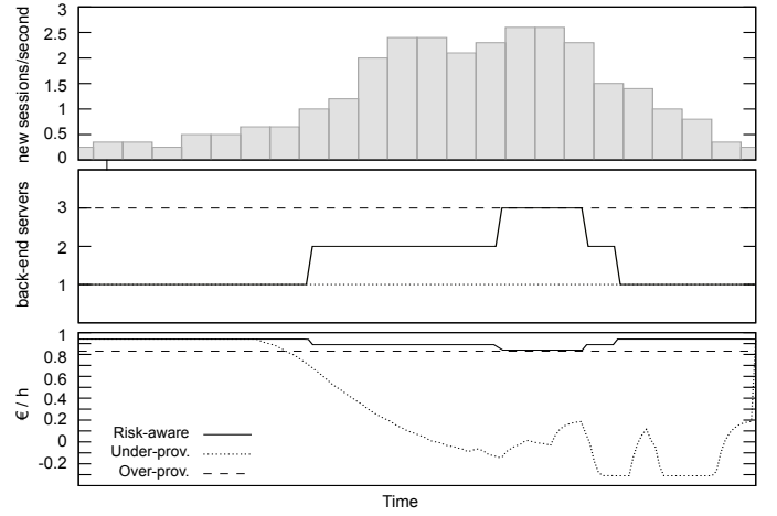
Fig. 4. CSP profit with a one-day typical workload.
