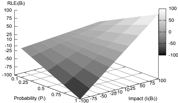
Fig. 2. Risk level estimations (in numeric values) of SEBCRA on BLOs.
